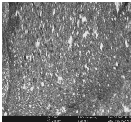
Fig. 5 SEM image of ZnO Nps-PVA-PEG-NF synthesized
