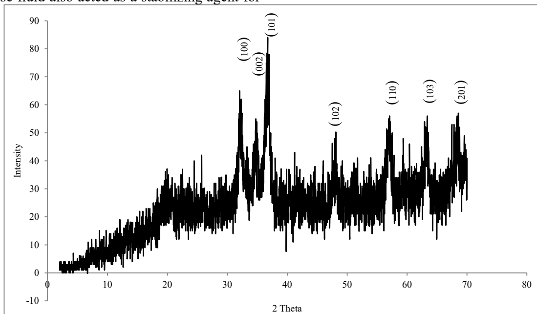
Fig. 3 XRD analysis of ZnO Nps-PVA-PEG-NF
