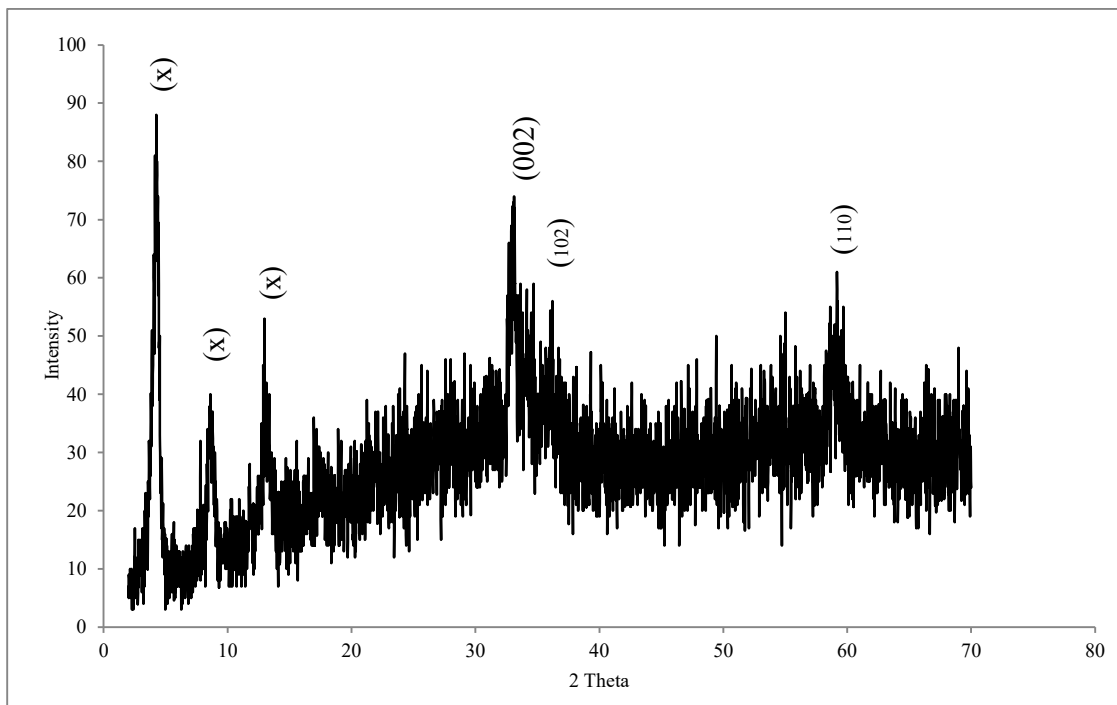
Fig. 4 XRD plot for ZnO Nps
